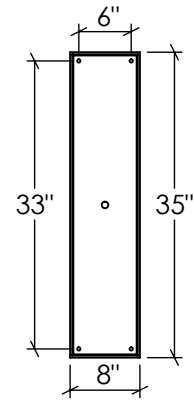
Backplate Mounting Detail Front View (Not to scale)
